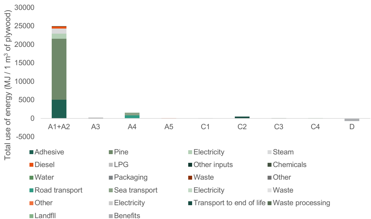
Figure 5- Contribution of main inputs and outputs of total energy use by module
