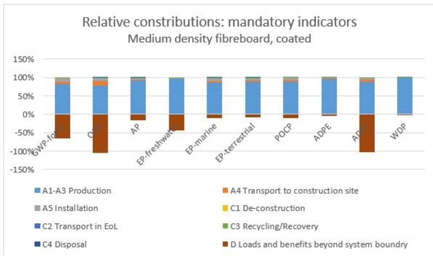
Figure 1: Environmental impacts of medium density fibreboard (MDF) coated with melamine-impregnated paper along its life cycle (impacts from production modules A1-C4 = 100 %)
